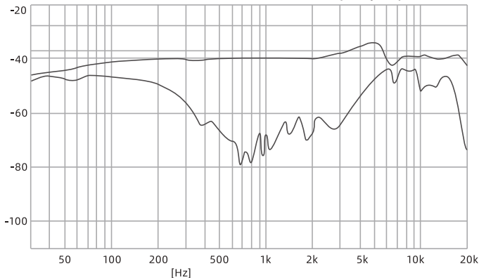
Frequency Response Curve
